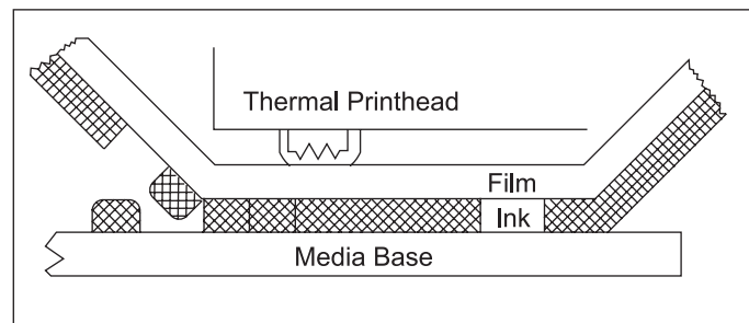
Figure 6. Thermal Transfer Printing
