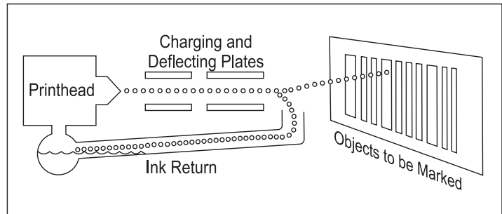
Figure 3. Ink Jet Printing
